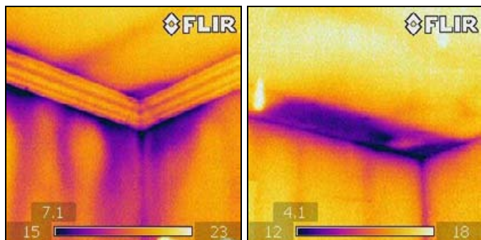
Above ▲ Uneven or limited insulation allows air to pass through wall and ceiling. Images taken in conjunction with a blower door test.
